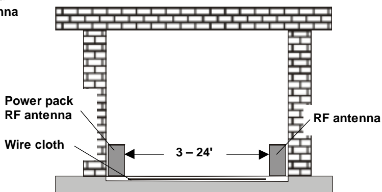
Figure 4. Pedestal with wire cloth
