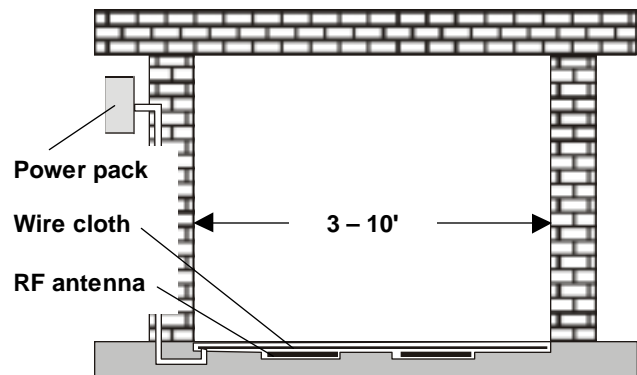
Figure 8. Sensormat II with wire cloth
