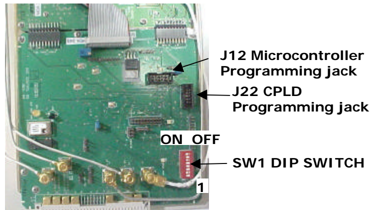
AGC Control Board, Axciter
