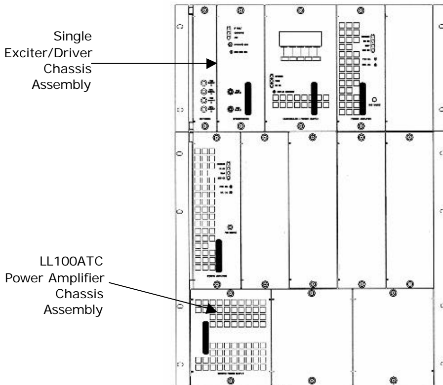
Figure 2-1: LL100ATC Front View
