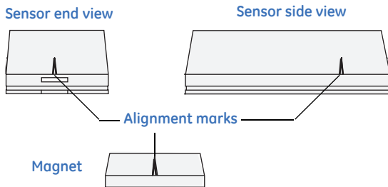
Figure 5. Alignment marks
