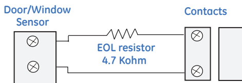
Figure 8. External contact wiring
