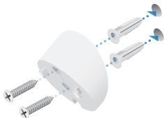
Angle Mount
