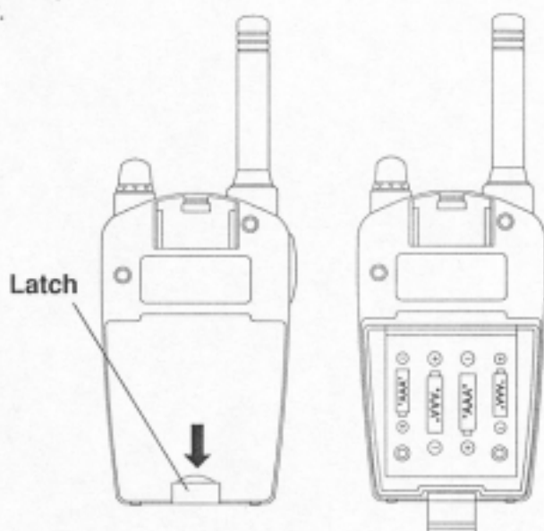
Figure 1 (Rear View)
