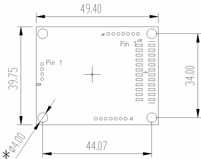
Figure 2-1 Dimensions of UIC6811
