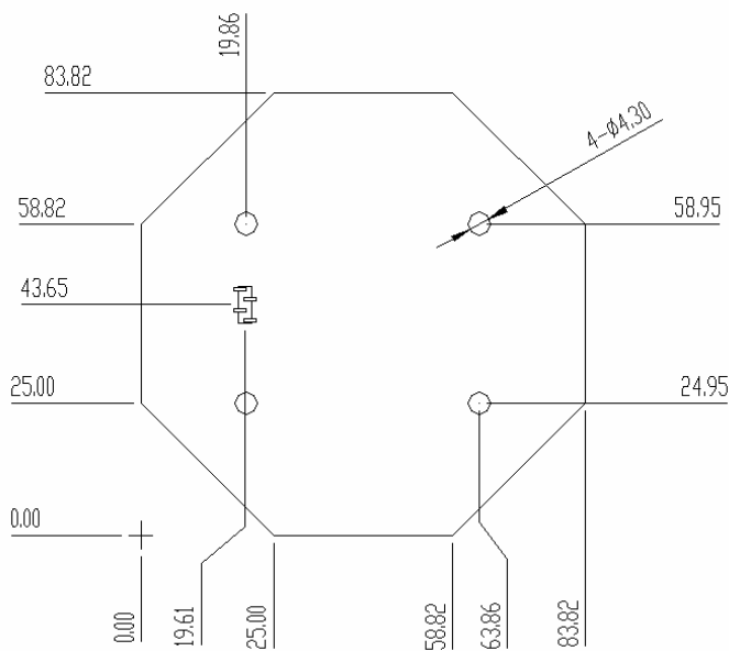
Figure 2-2 Dimensions of Remote Antenna PCBA
