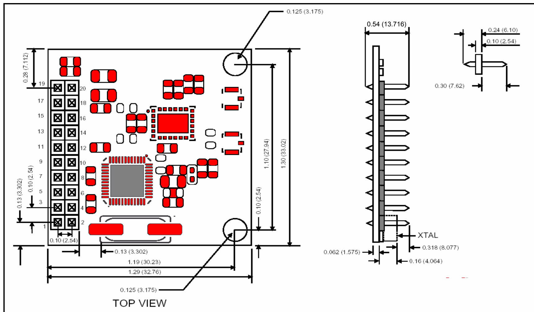
Figure 3 – Juno-LPA Dimensions
