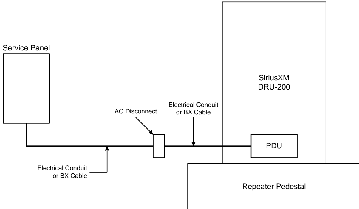
Figure 3-37 AC Power Cable Routing
