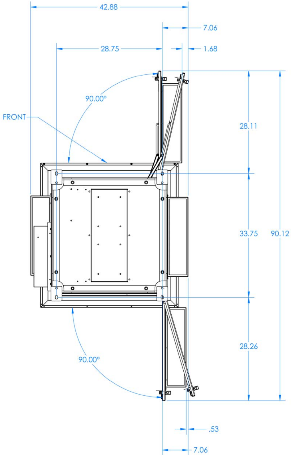
Figure 3-2 Repeater Cabinet Bottom Up View
