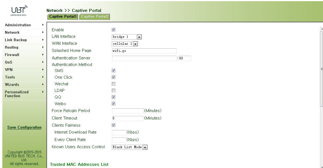
Figure 3-38 Captive Portal
