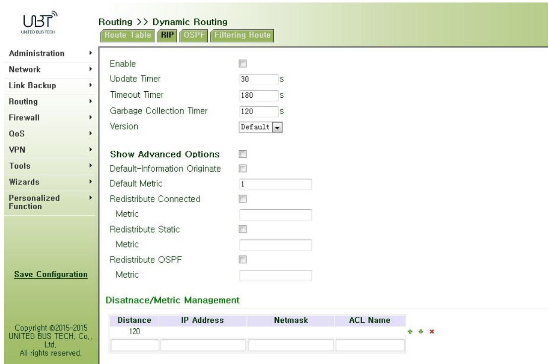
Figure 3-59-2 RIP
