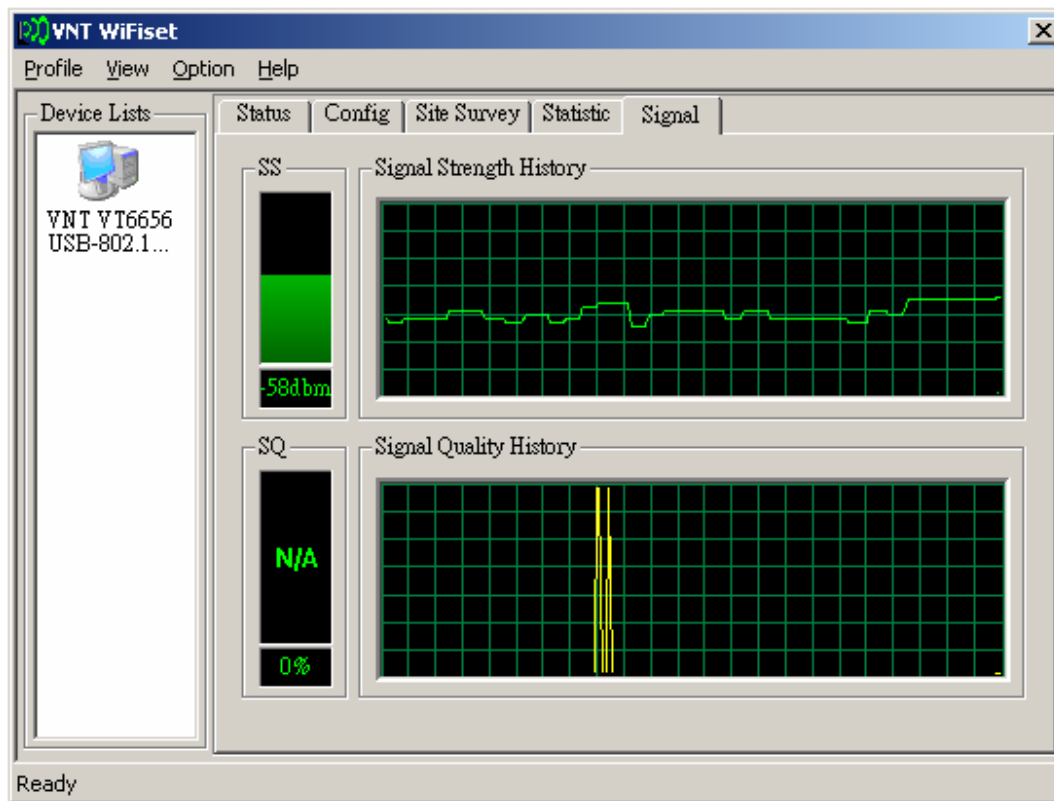
Figure 7. WiFiset—Signal
