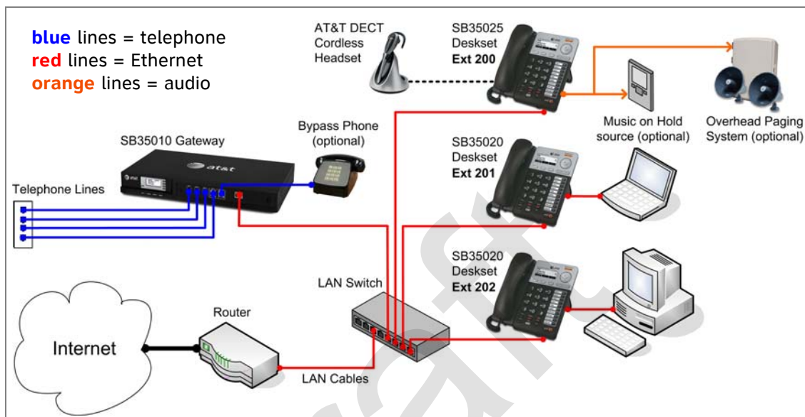
Figure 1. Sample Syn248 System
