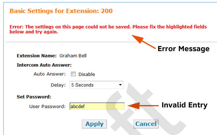
Figure 27. WebUI Error Indication
