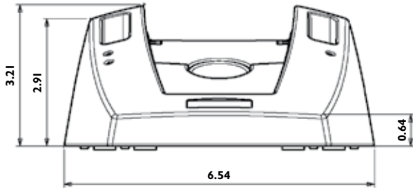
Front view - dimensions in inches
