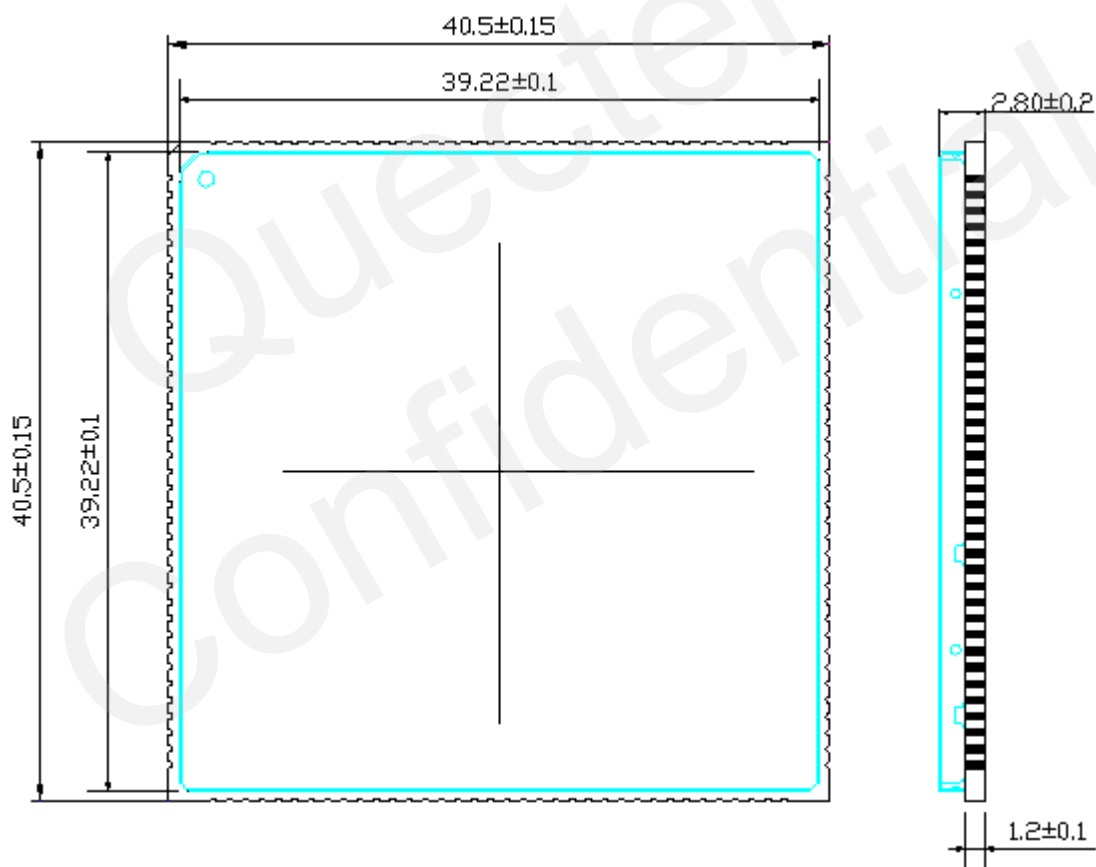
Figure 3: Module Top and Side Dimensions
