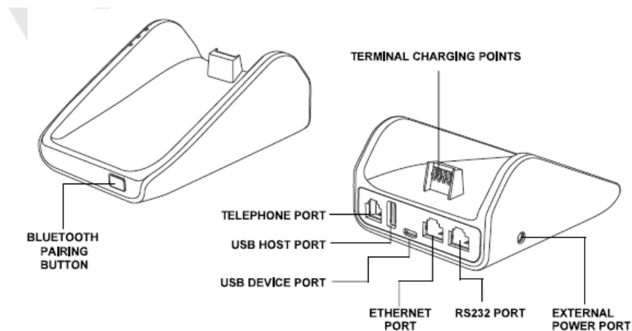
Figure 4 V400m FF Base, Front and Rear
