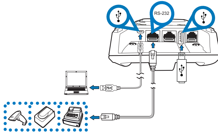
Figure 18 Connecting Peripheral Devices
