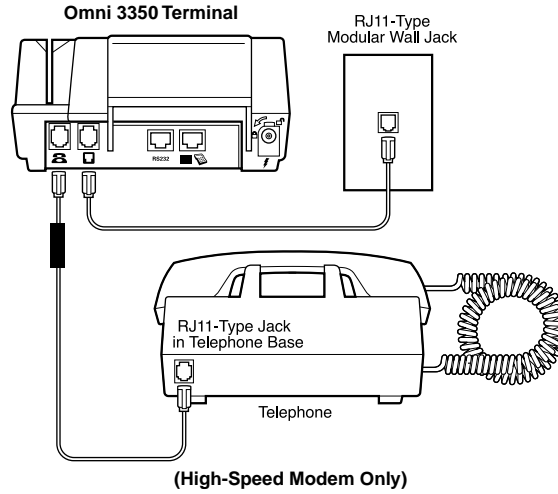
Figure 5 Pass-Through Connection
