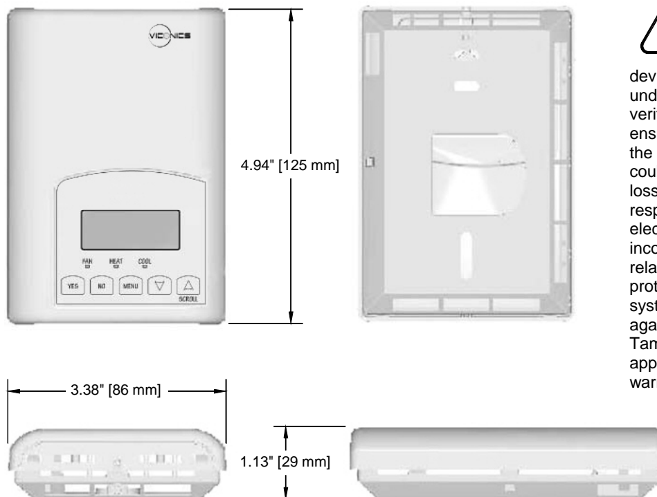
Fig. 13 – Thermostat dimensions
