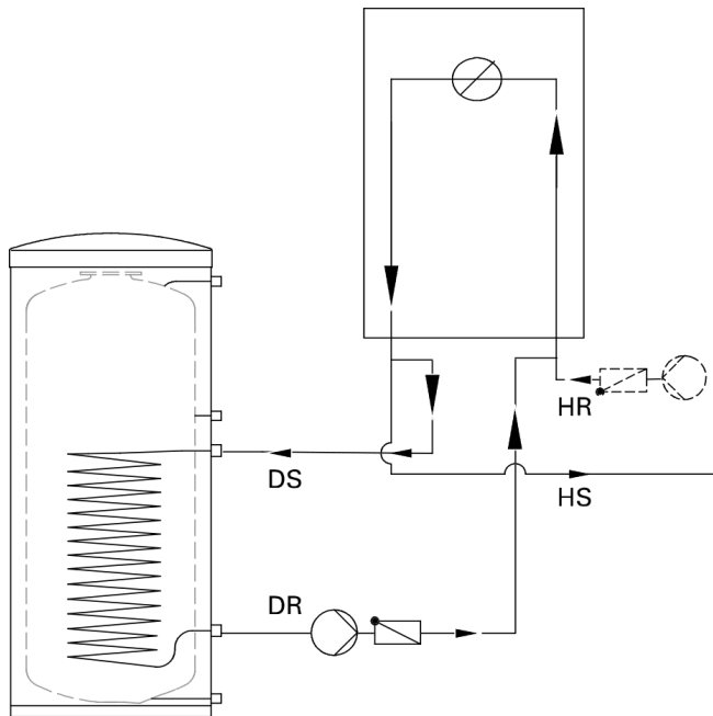
Connections for model B2HA 100
