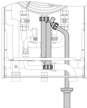
Condensate Connection for Vitodens 200-W, models B2HA 100
