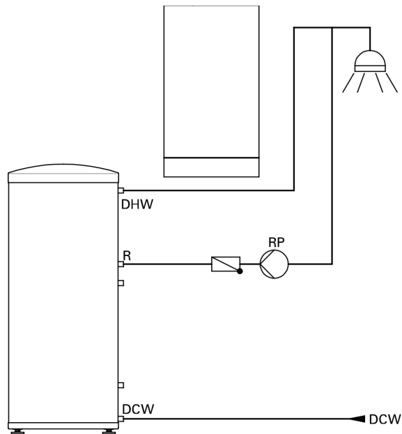
Vitocell-V stand-alone DHW storage tank
