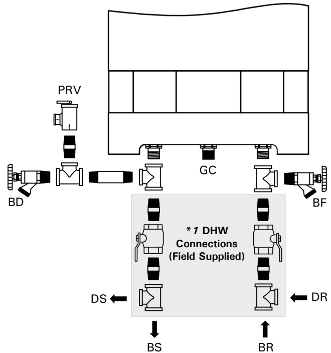
Connections for model B2HA 100
