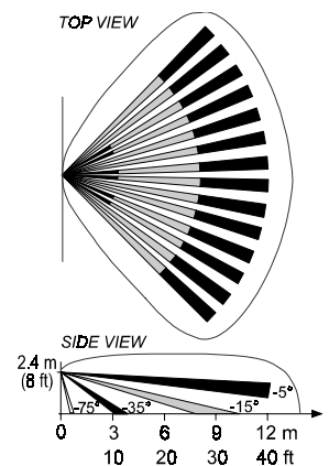
Figure 2. PIR and MW Coverage Pattern
