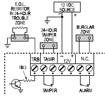
Figure 5. Terminal Block Wiring
