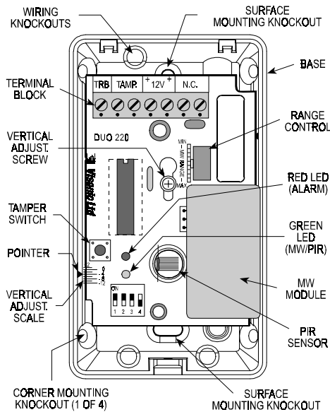
Figure 3. Printed Circuit Board Layout
