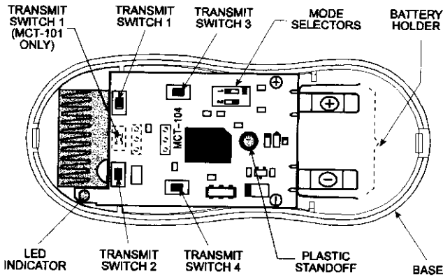
Figure 3. Component Layout
