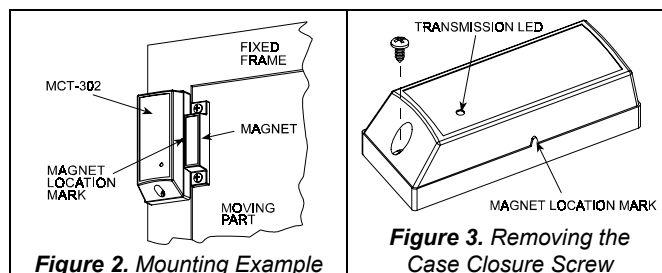
Figure 2. Mounting Example
