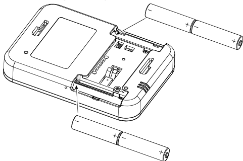
Figure 1 – Battery Insertion
