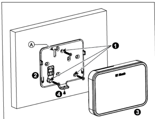
Figure 4 – Wall Mounting
