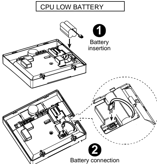
Figure 10. Battery Replacement
