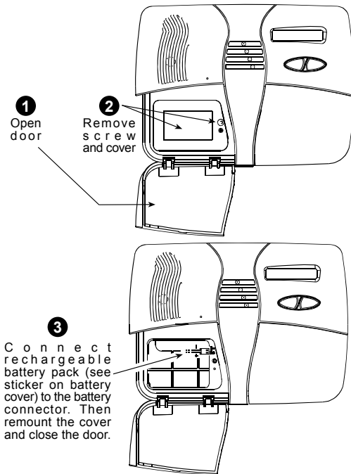
Figure 10. Battery Replacement
