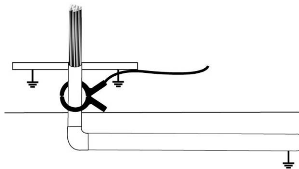
Inductive Coupling with the signal clamp
