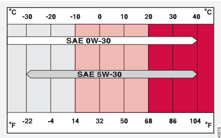
Viscosity chart
