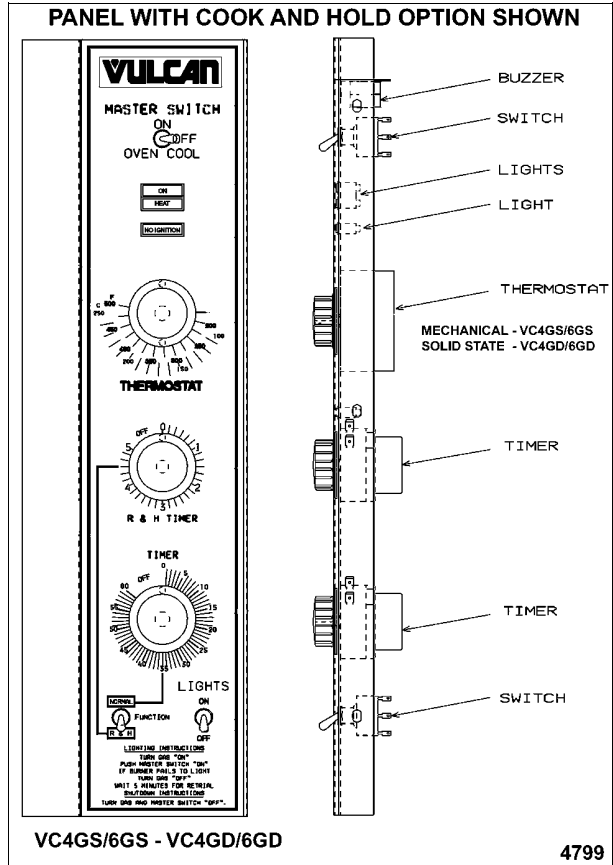
PANEL WITH COMPUTER CONTROL SHOWN
