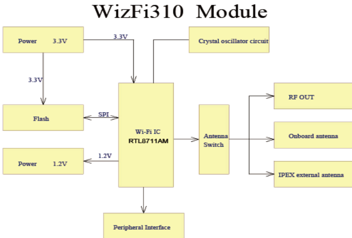
Figure 3-1 WizFi310 System Diagram
