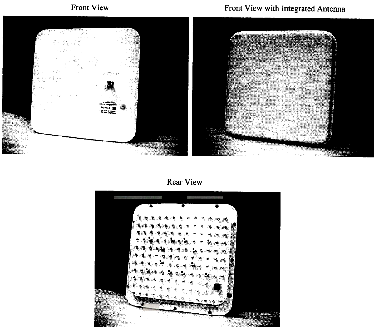
Figure 1. Wireless Transceiver
