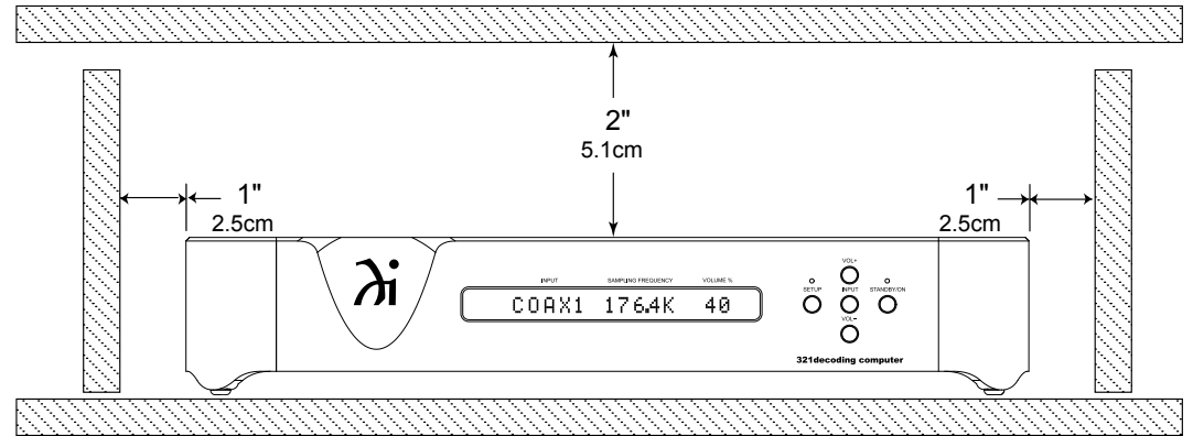
321 Front View
