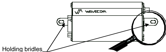
Figure 2 Modem mounting
