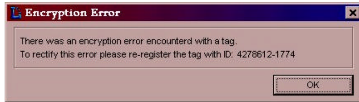
Figure 26: Encryption Error
