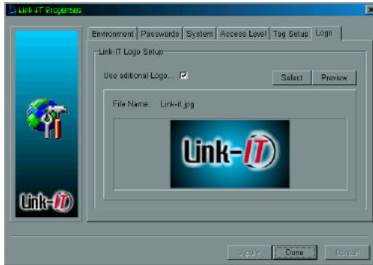
Figure 25: Logo Setup
