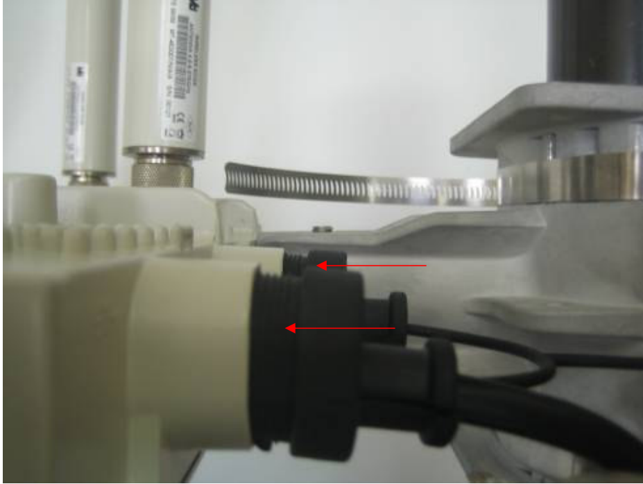
Figure 4.12 Sealing rubber
