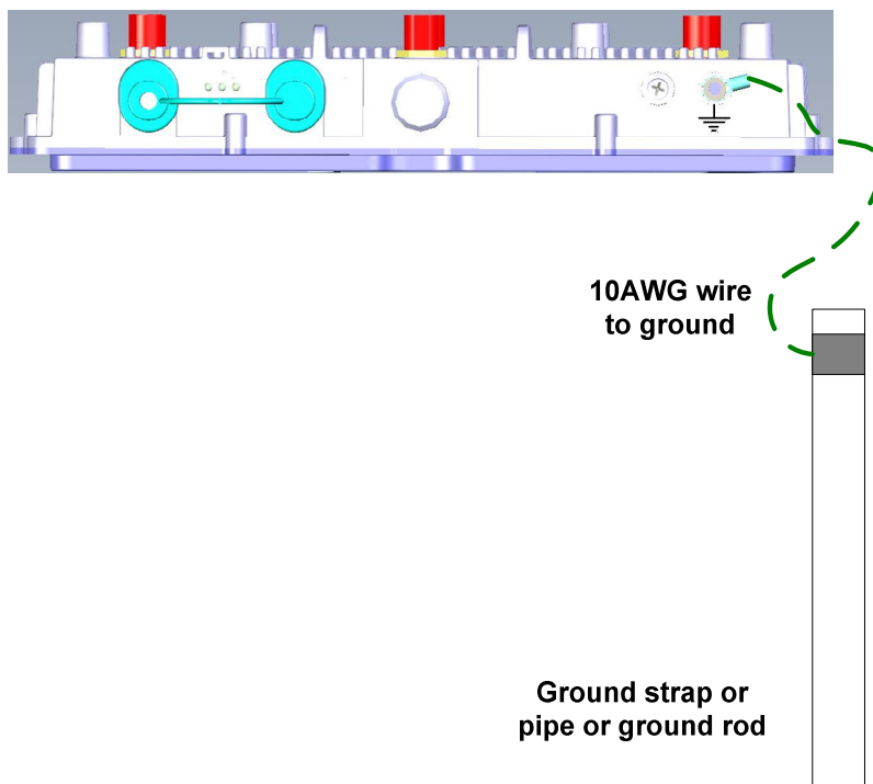
Figure 4.6 Grounding Method
