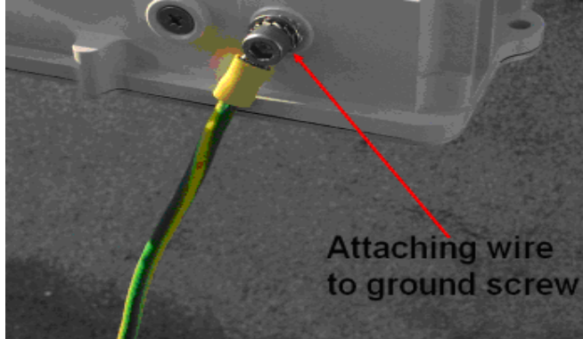
Figure 4.7 Grounding
