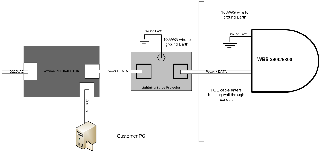
Figure 4.8 Grounding indoor injector by Network Protection Unit
