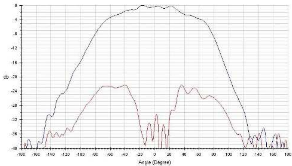
Single port azimuth radiation pattern including cross-pol at 5.8GHz
