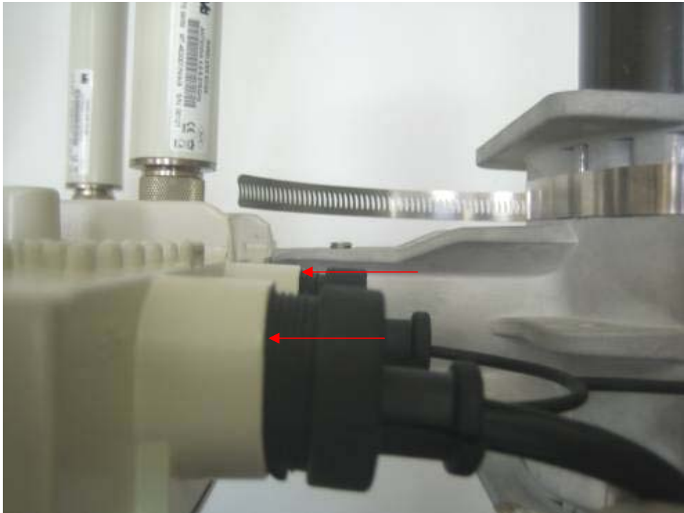
Figure 4.12 Sealing rubber
