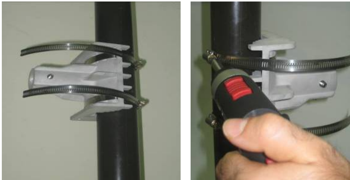
Figure 4.3 Using Special Hose Clamps & Screwing the Clamps
