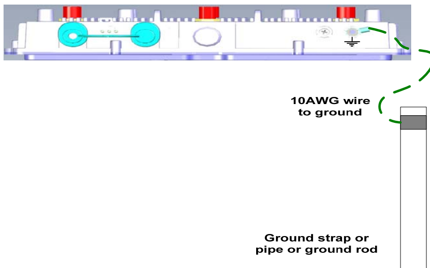
Figure 4.6 Grounding Method
