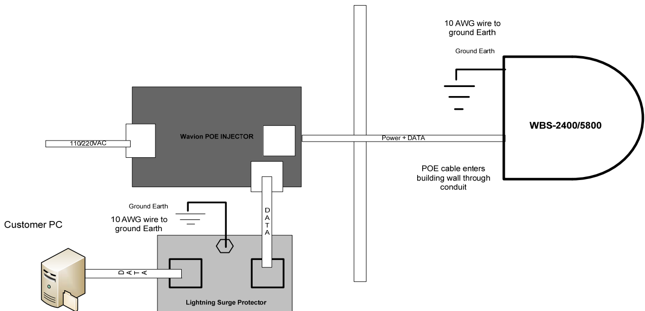
Figure 4.8 Grounding indoor injector by Network Protection Unit
