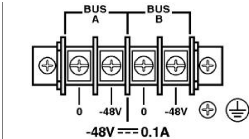
Figure 4.1: Terminal Block Assembly (DC Units Only)
