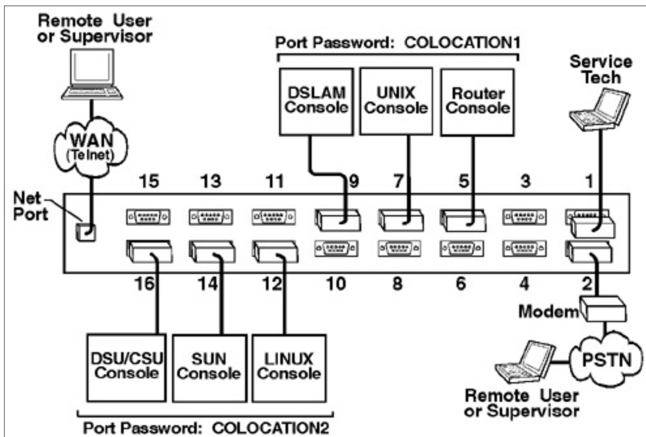
Figure 4.2: CMS Application Example (Not to Scale)
