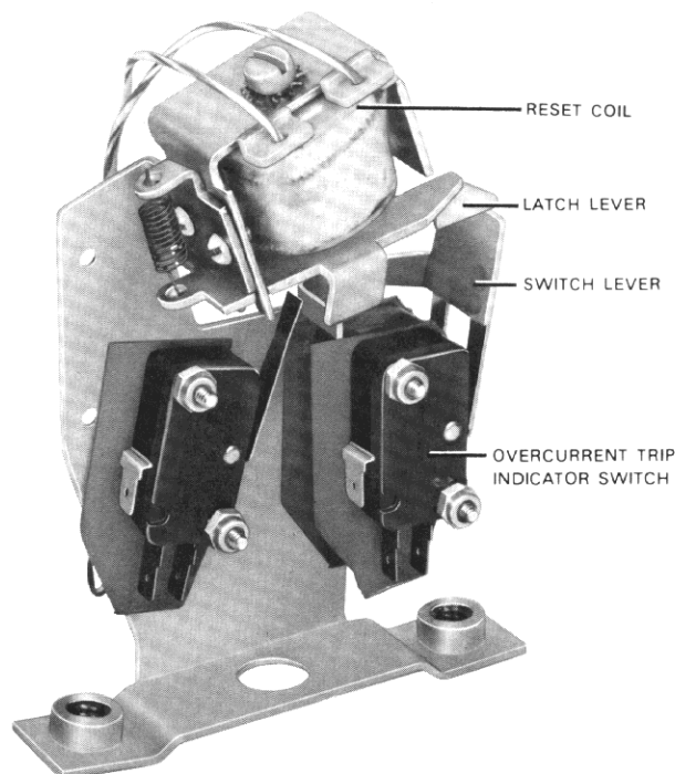
Fig. 31 Overcurrent Trip Switch
