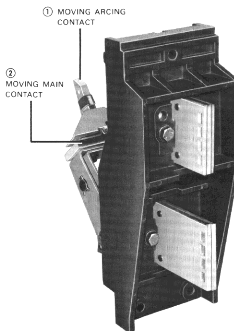
Fig. 6 Type DS-416 Pole Unit Assembly—Rear View
