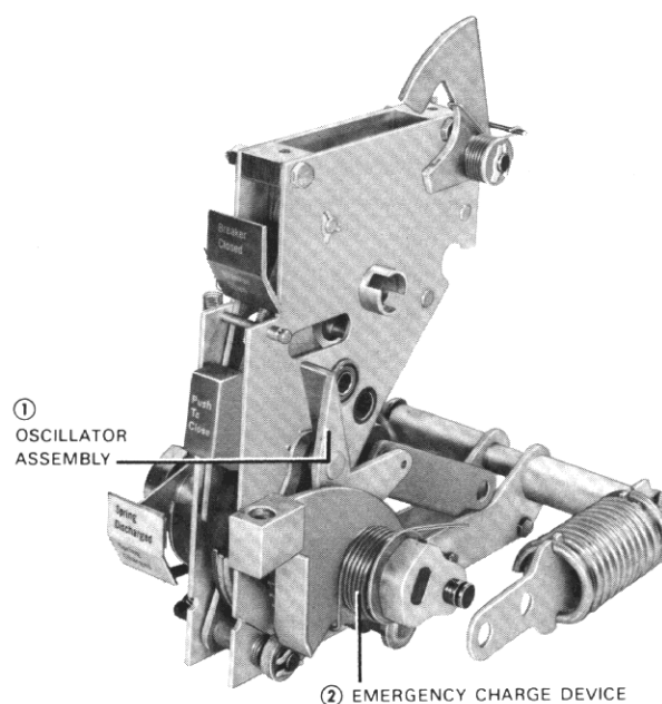
Fig. 20 Front View of Mechanism (Power-Operated Spring Charge)
