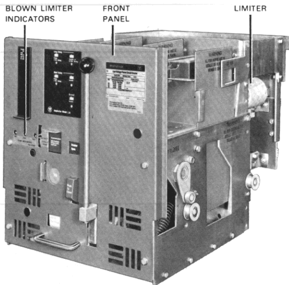
Fig. 32 DSL-206 Breaker—Front View
