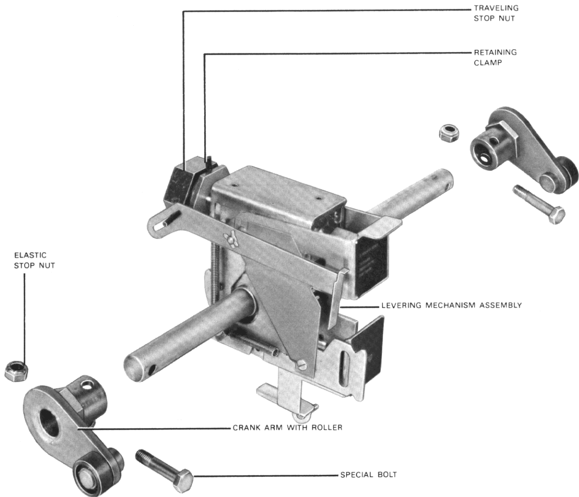
Fig. 18 Levering Mechanism
