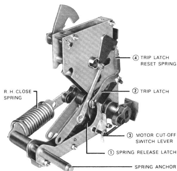
Fig. 22 Rear View of Power-Operated Mechanism (Left Close Spring Removed)
