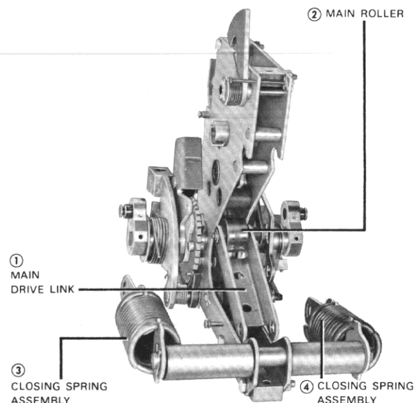
Fig. 21 Rear of Power-Operated Mechanism
