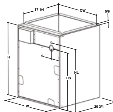
Figure 1. Cased Coil
