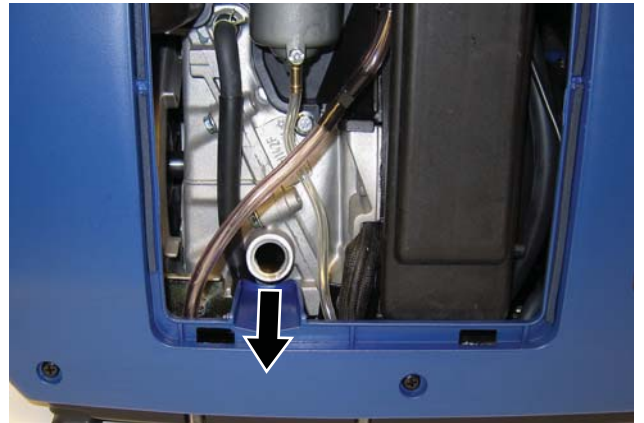
Figure 39 – Draining Engine Oil
