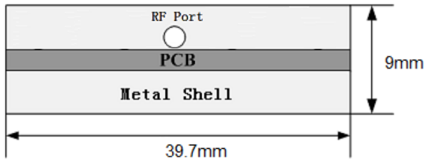
Drawing2 Side view of the reader
