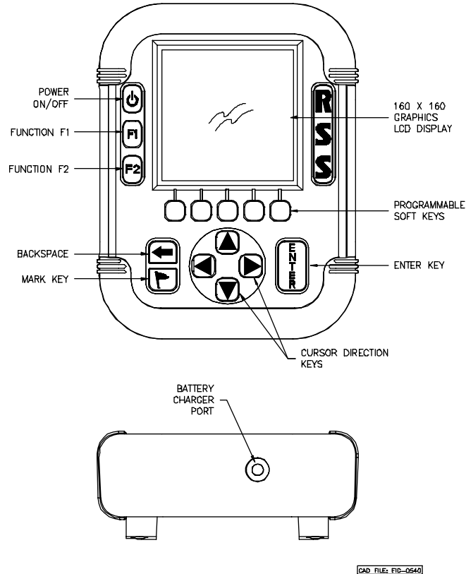
Figure 4. Remote Features
