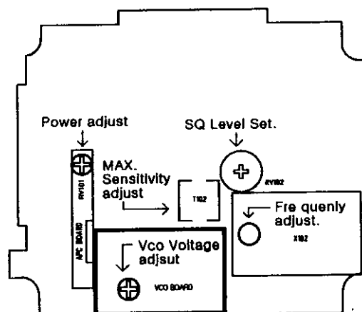
[ RF SECTION ]
