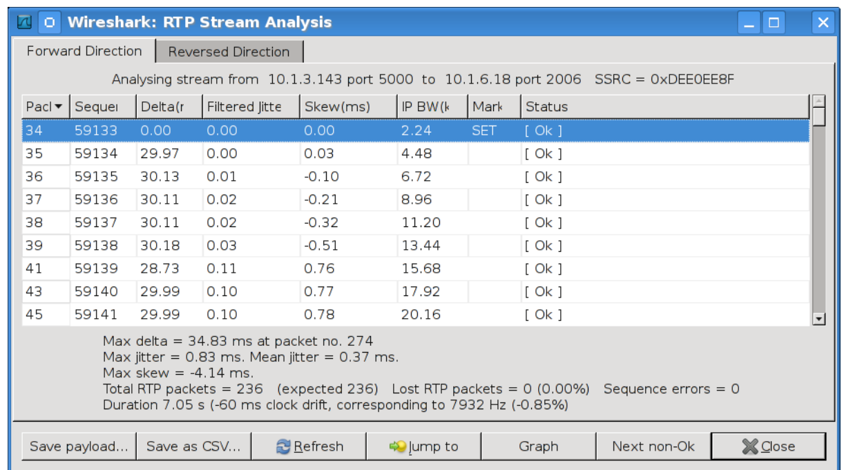
Figure 9.1. The "RTP Stream Analysis" window
