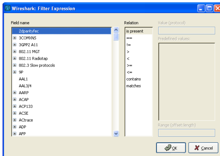
Figure 6.7. The "Filter Expression" dialog box
