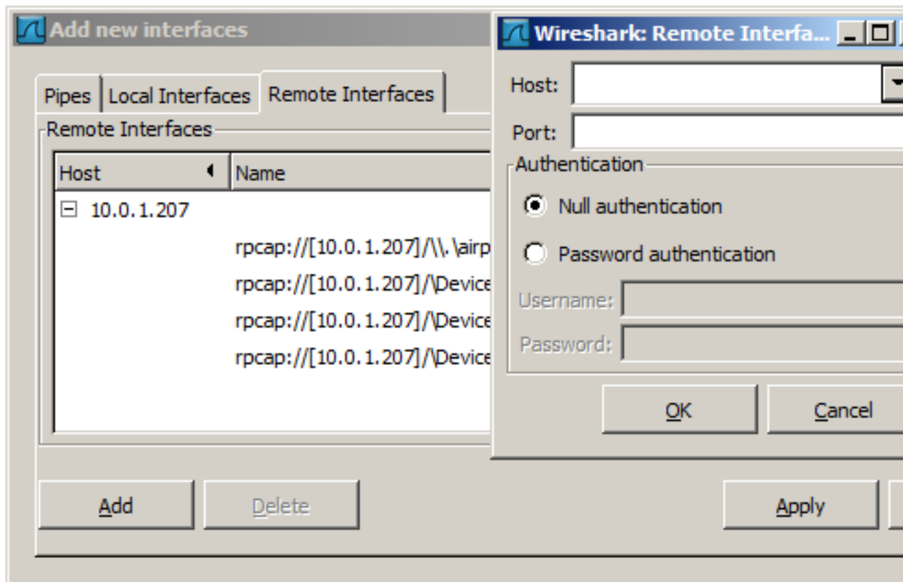
Figure 4.9. The "Remote Capture Interfaces" dialog box
