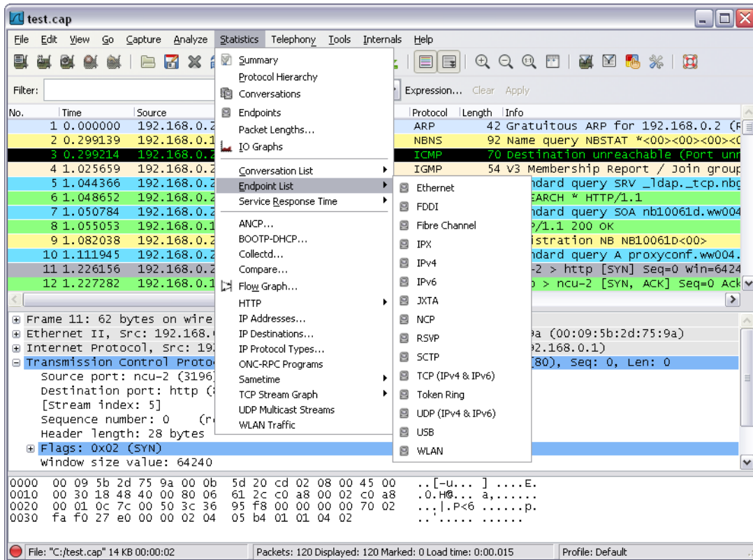
Figure 3.9. The "Statistics" Menu
