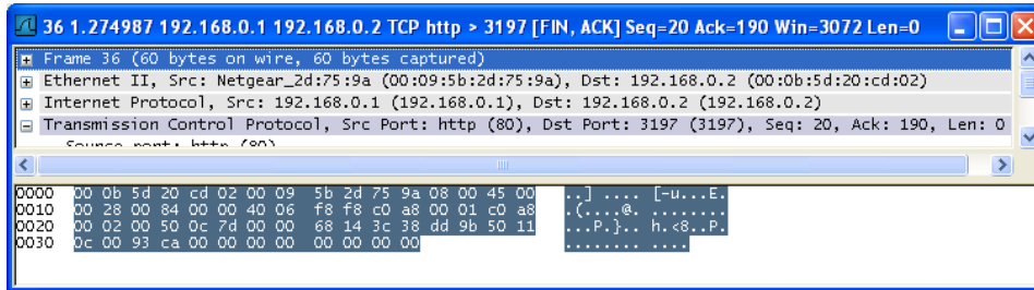
Figure 6.2. Viewing a packet in a separate window
