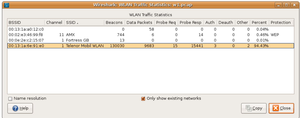
Figure 8.9. The "WLAN Traffic Statistics" window
