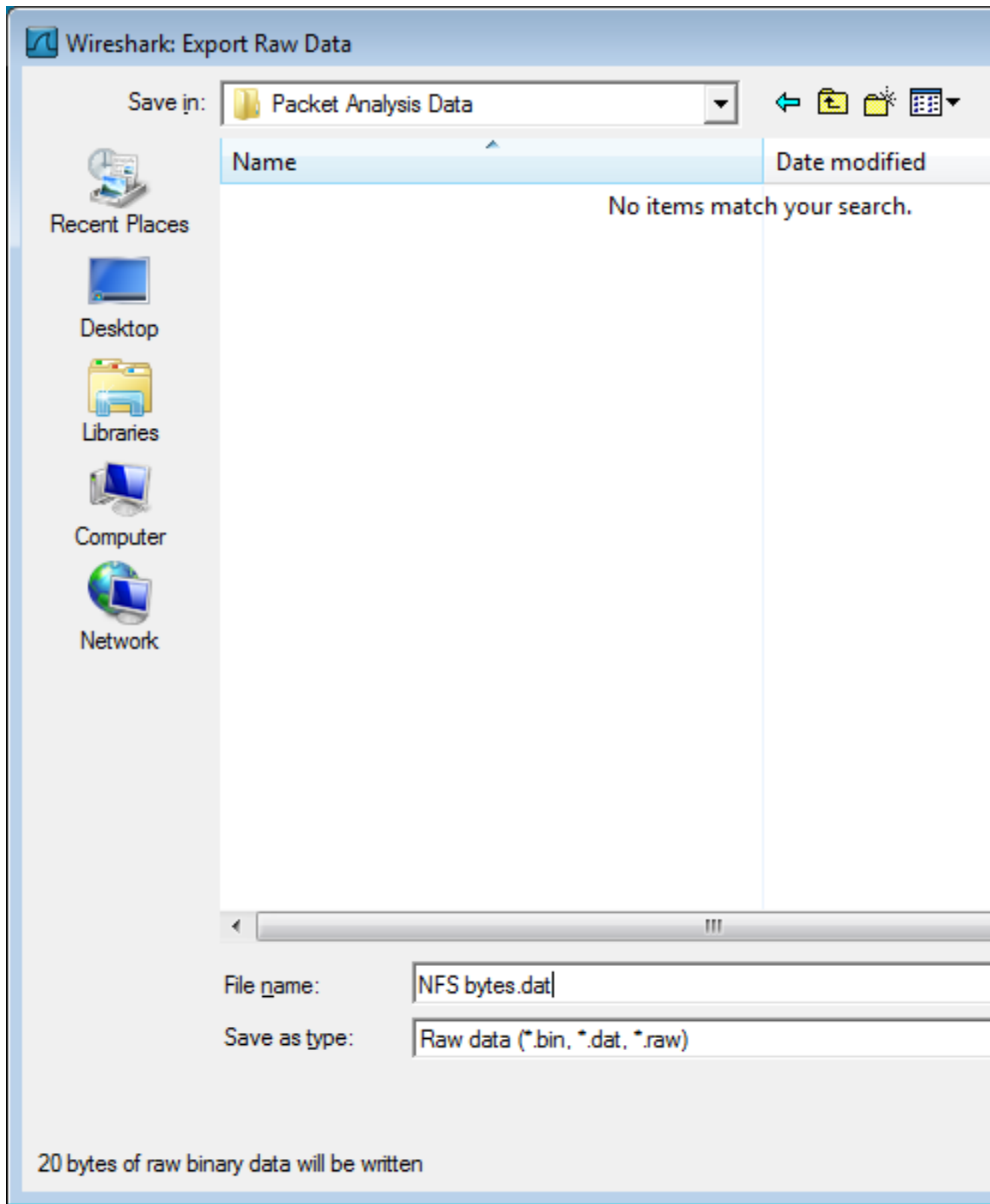
Figure 5.16. The "Export Selected Packet Bytes" dialog box
