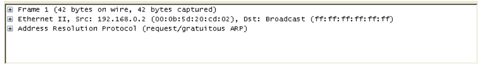
Figure 3.17. The "Packet Details" pane
