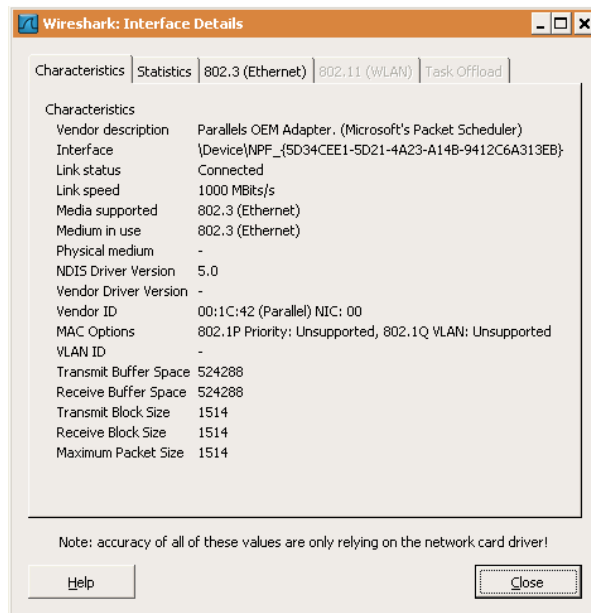
Figure 4.11. The "Interface Details" dialog box
