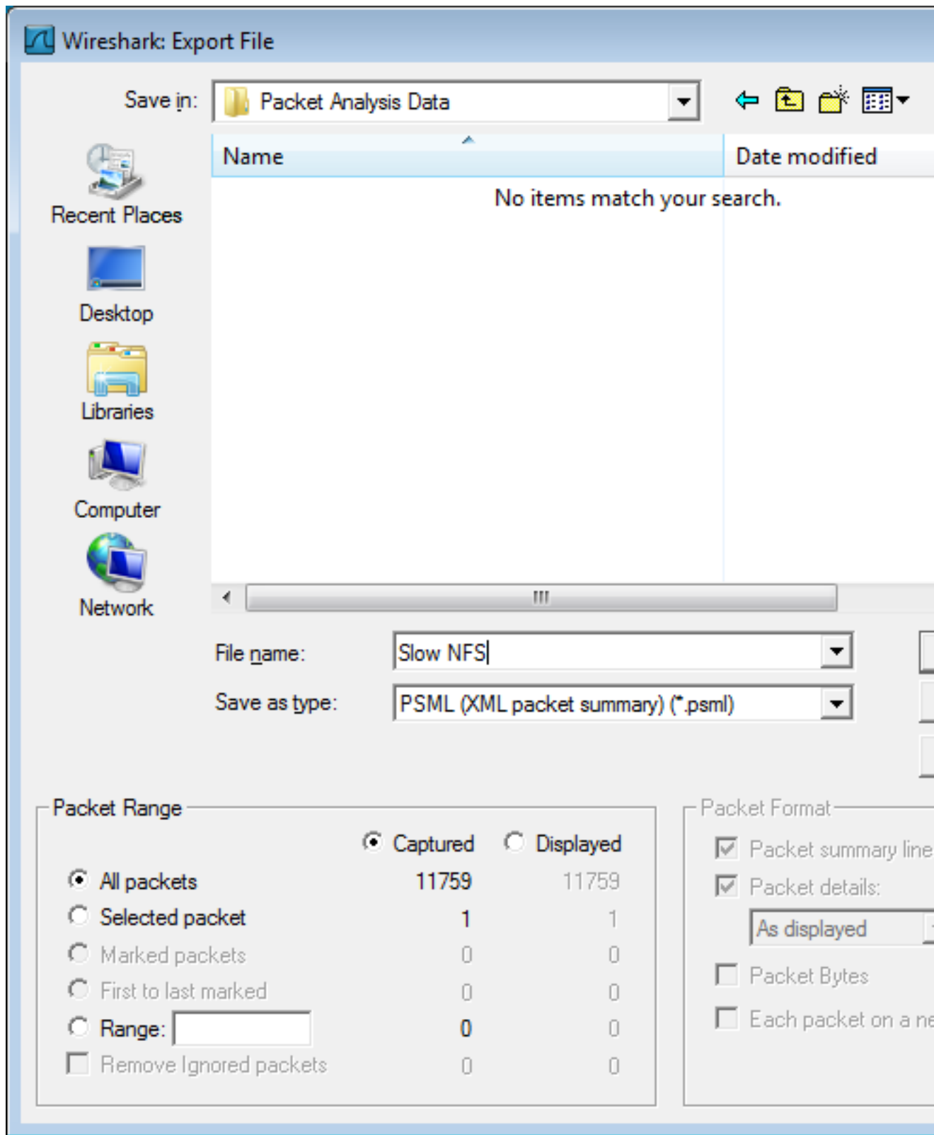
Figure 5.14. The "Export as PSML File" dialog box
