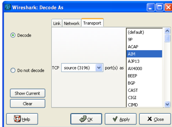
Figure 10.6. The "Decode As" dialog box
