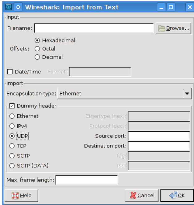
Figure 5.10. The "File Import" dialog
