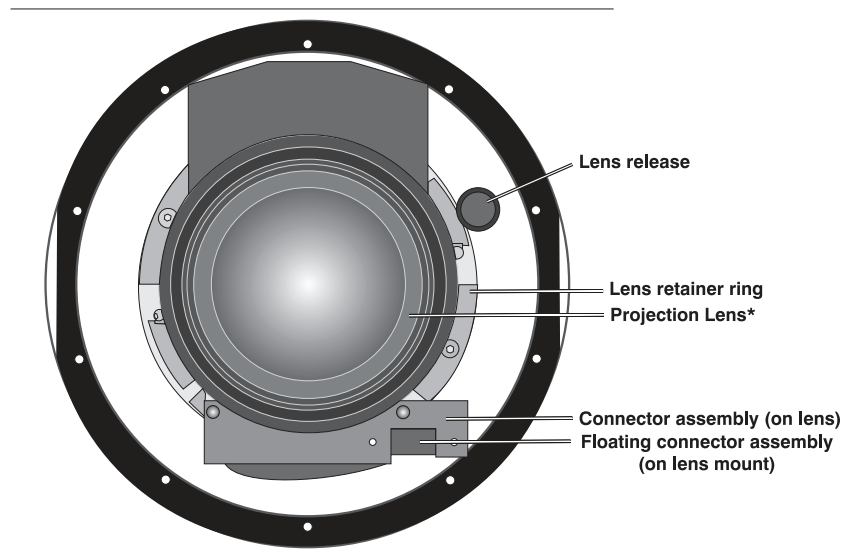
Figure 4.8. Lens Assembly
