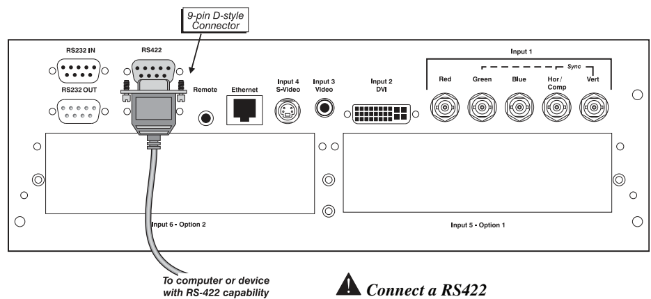
Figure 2.11 Connecting RS-422
