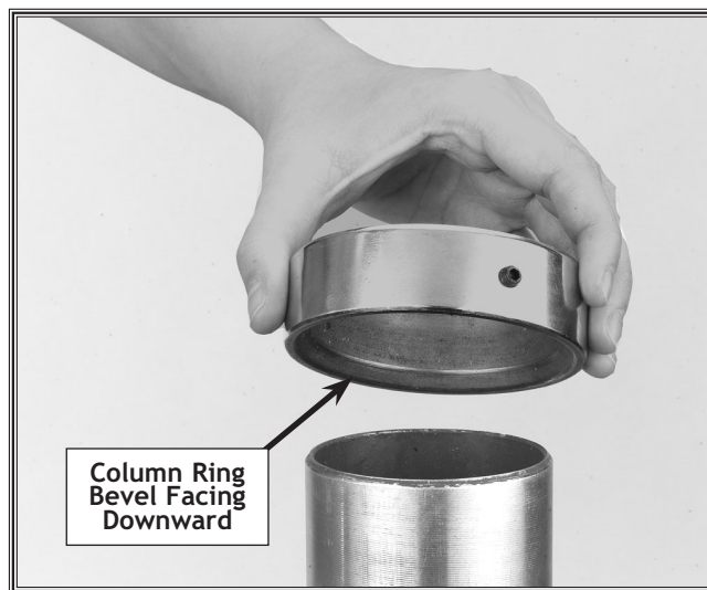
Figure 14. Column ring bevel positioning.
