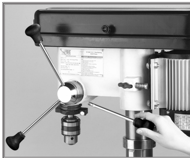
Figure 21. Installing spindle handles.
