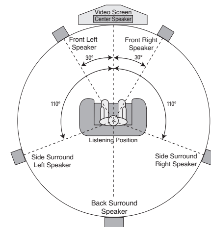
6.1 Placement Diagram
