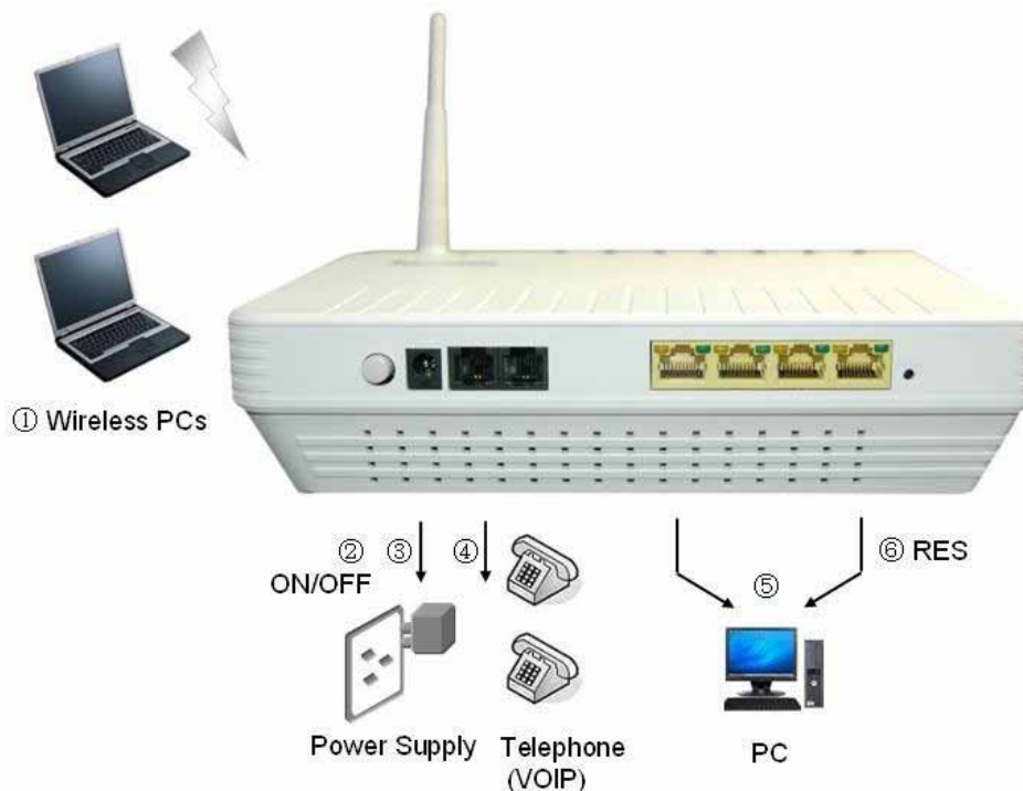
Figure 4: Overview of Hardware Connections for FG101
