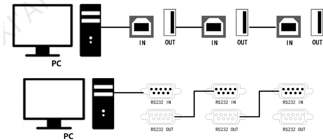
Fig. 3-2 Multiple 3D HD cascade
